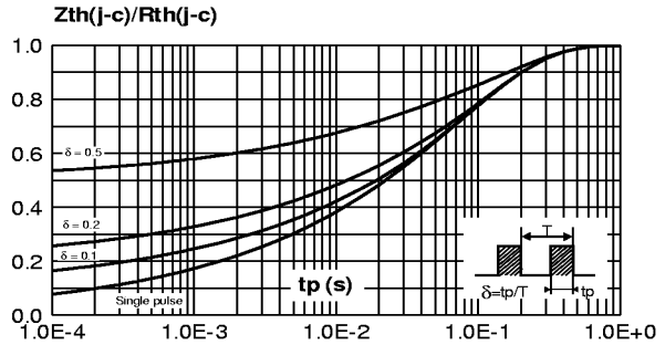
Fig. 4: Relative variation of thermal impedance junction to case versus pulse duration.
