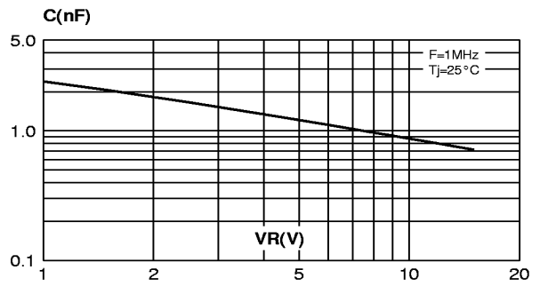
Fig. 6: Junction capacitance versus reverse voltage applied (typical values).
