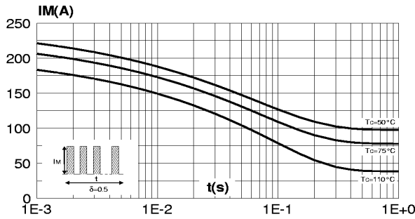
Fig. 3: Non repetitive surge peak forward current versus overload duration (maximum values).
